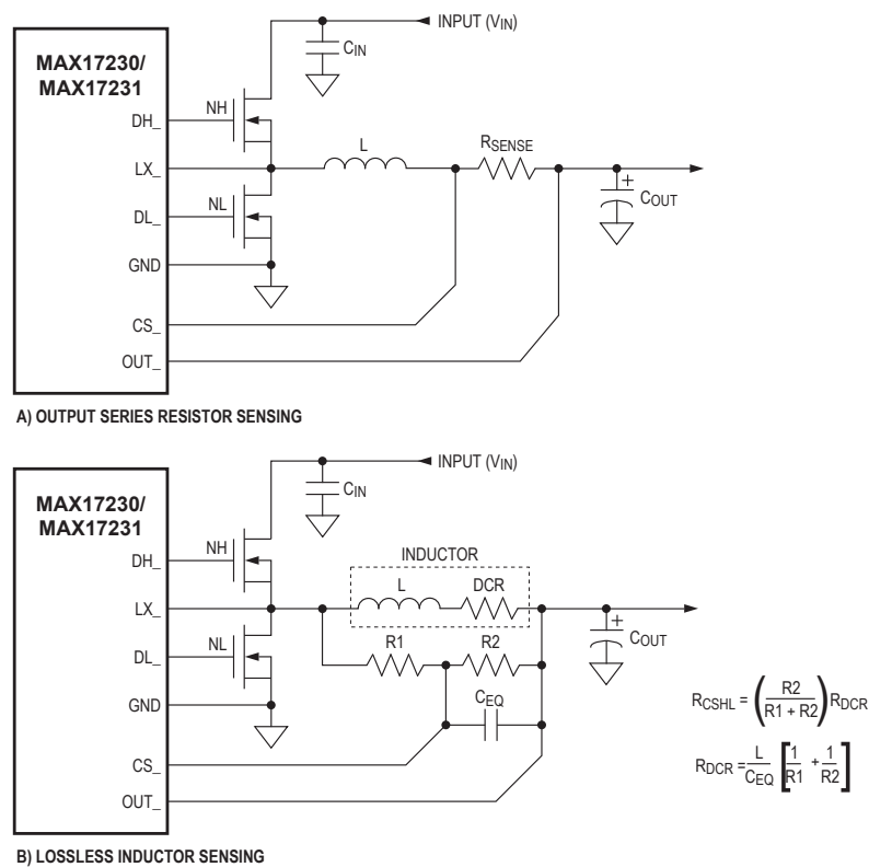
Figure 1. Current-Sense Configurations
