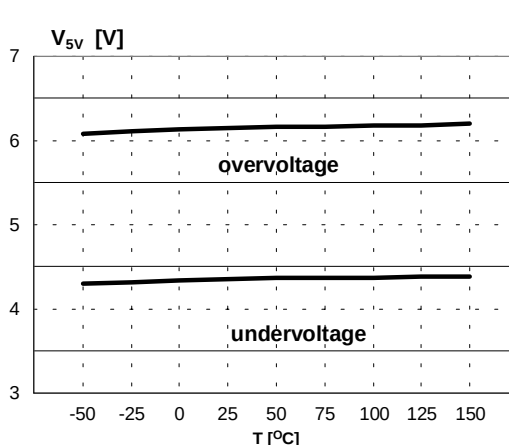
Figure 6. 5V fault thresholds
