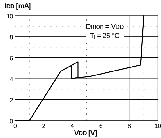
Figure 2. IC Supply current vs. supply voltage
