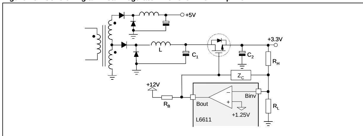
Figure 24. Auxiliary OVP without Crowbar
