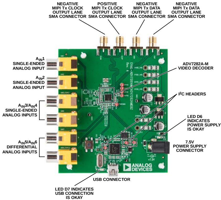
Figure 3. ADV7282A-M. Evaluation Board
