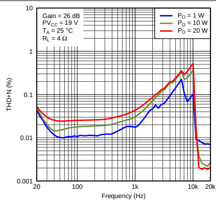
Figure 10. Total Harmonic Distortion + Noise (TPA3132D2 PBTL) vs Frequency
