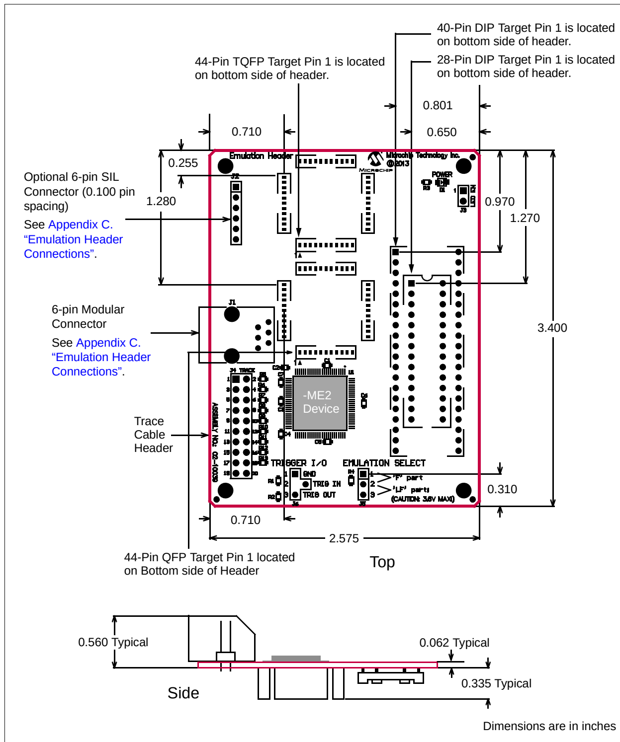
FIGURE 3-1: DIMENSIONS - AC244055
