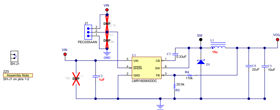
Figure 5. LMR1606XEVM Schematic
