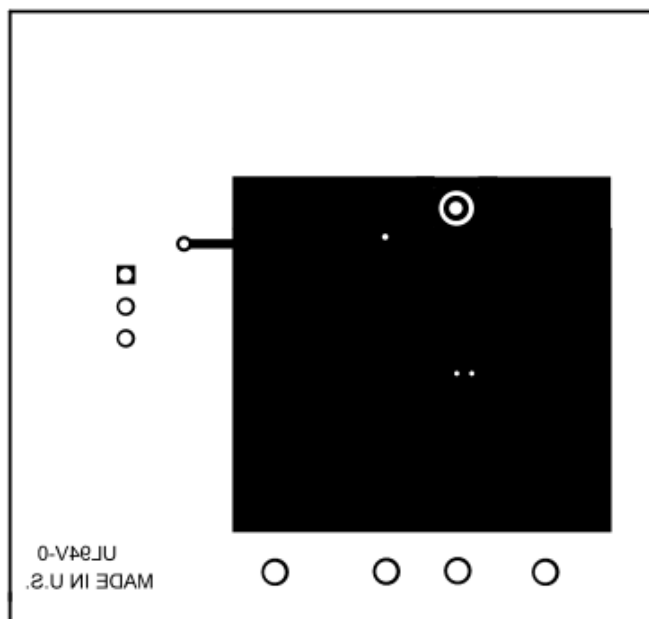
Figure 4. Bottom Layer
