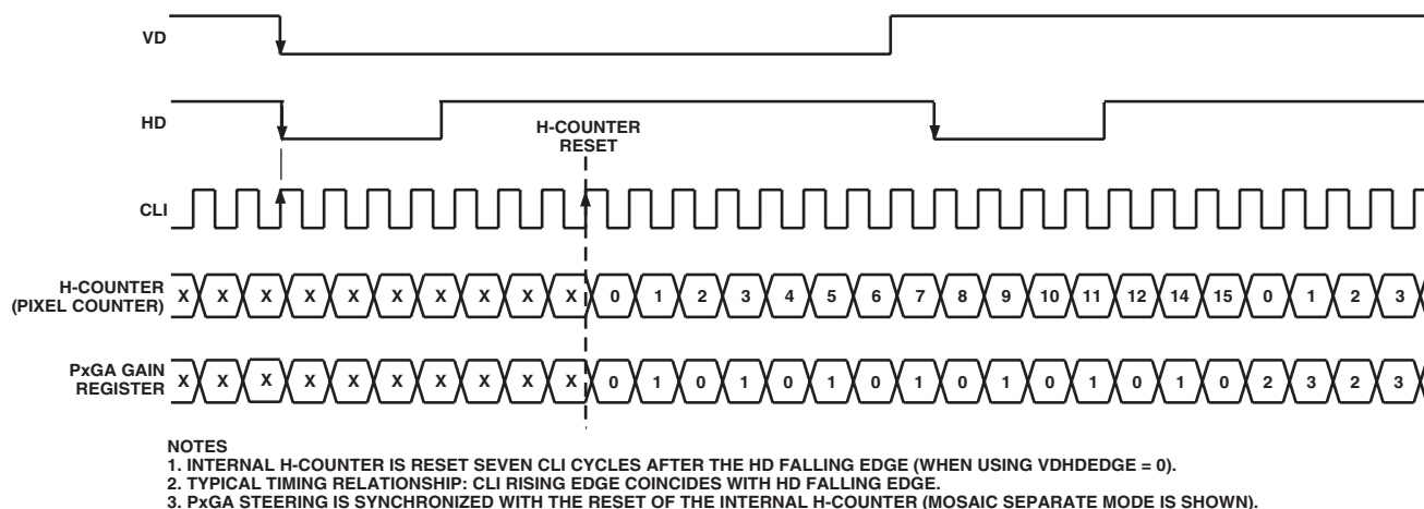
Figure 13. H-Counter Synchronization
