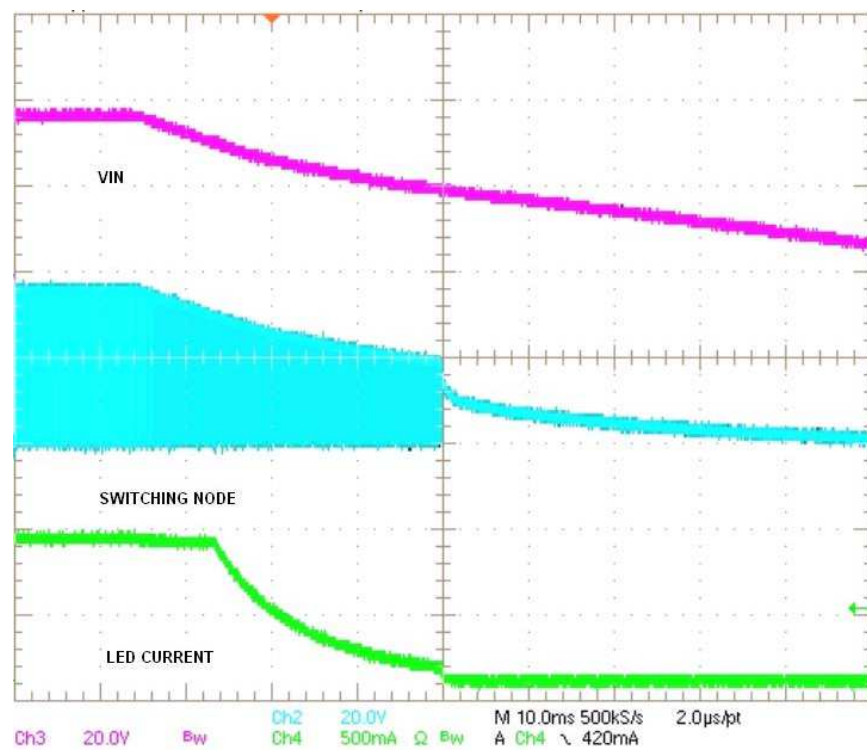
Figure 12. Buck Converter Shut-Down Waveform
