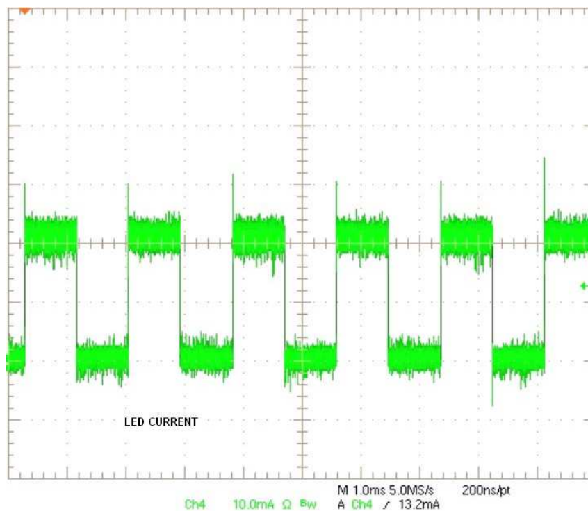
Figure 10. TPS92660EVM Linear Regulator PWM Dimming, L ADJ = 1.25 V
