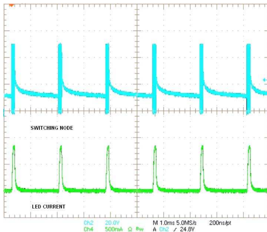
Figure 9. TPS92660EVM Buck Converter PWM Dimming, S ADJ = 0.25 V
