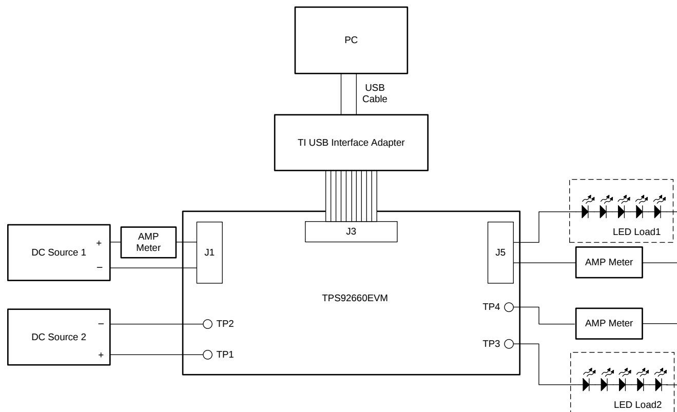
Figure 2. TPS92660EVM Recommended Test Set Up
