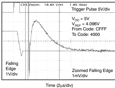
Figure 16. Half-Scale Settling Time: 5-V Falling Edge
