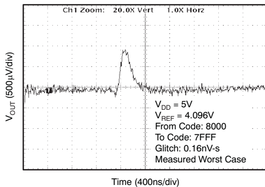
Figure 18. Glitch Impulse: 5 V, 1-LSB Step, Falling Edge
