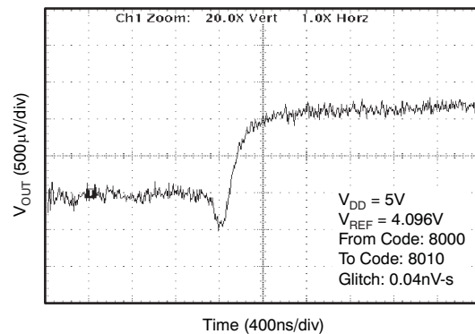
Figure 19. Glitch Impulse: 5 V, 16-LSB Step, Rising Edge
