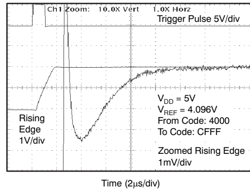
Figure 15. Half-Scale Settling Time: 5-V Rising Edge
