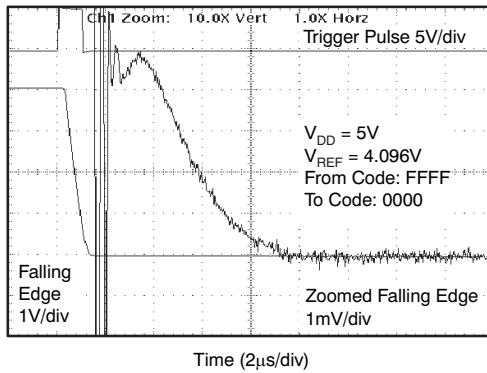
Figure 14. Full-Scale Settling Time: 5-V Falling Edge
