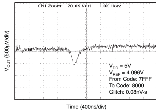
Figure 17. Glitch Impulse: 5 V, 1-LSB Step, Rising Edge
