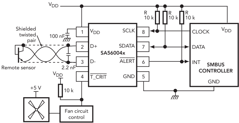
SA56004x system application diagram
