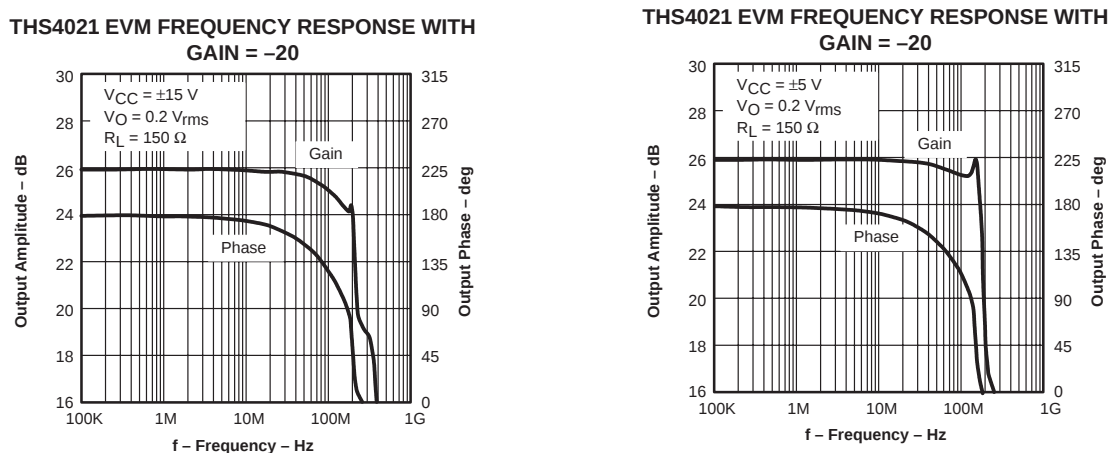
Figure 1–4. THS4021 EVM Frequency Response With Gain = -20
