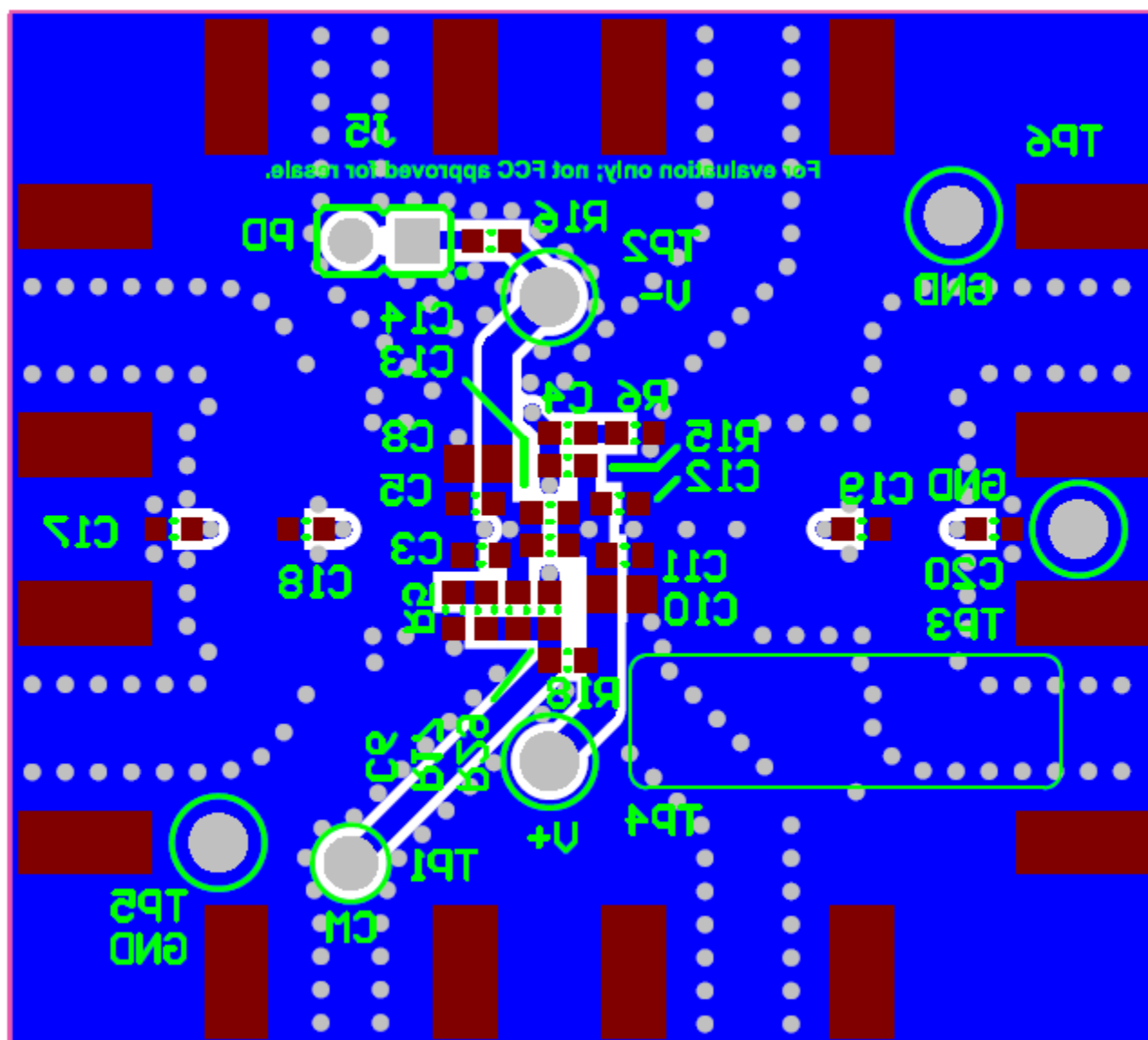
Figure 5. THS4551RUNEVM Bottom Layer
