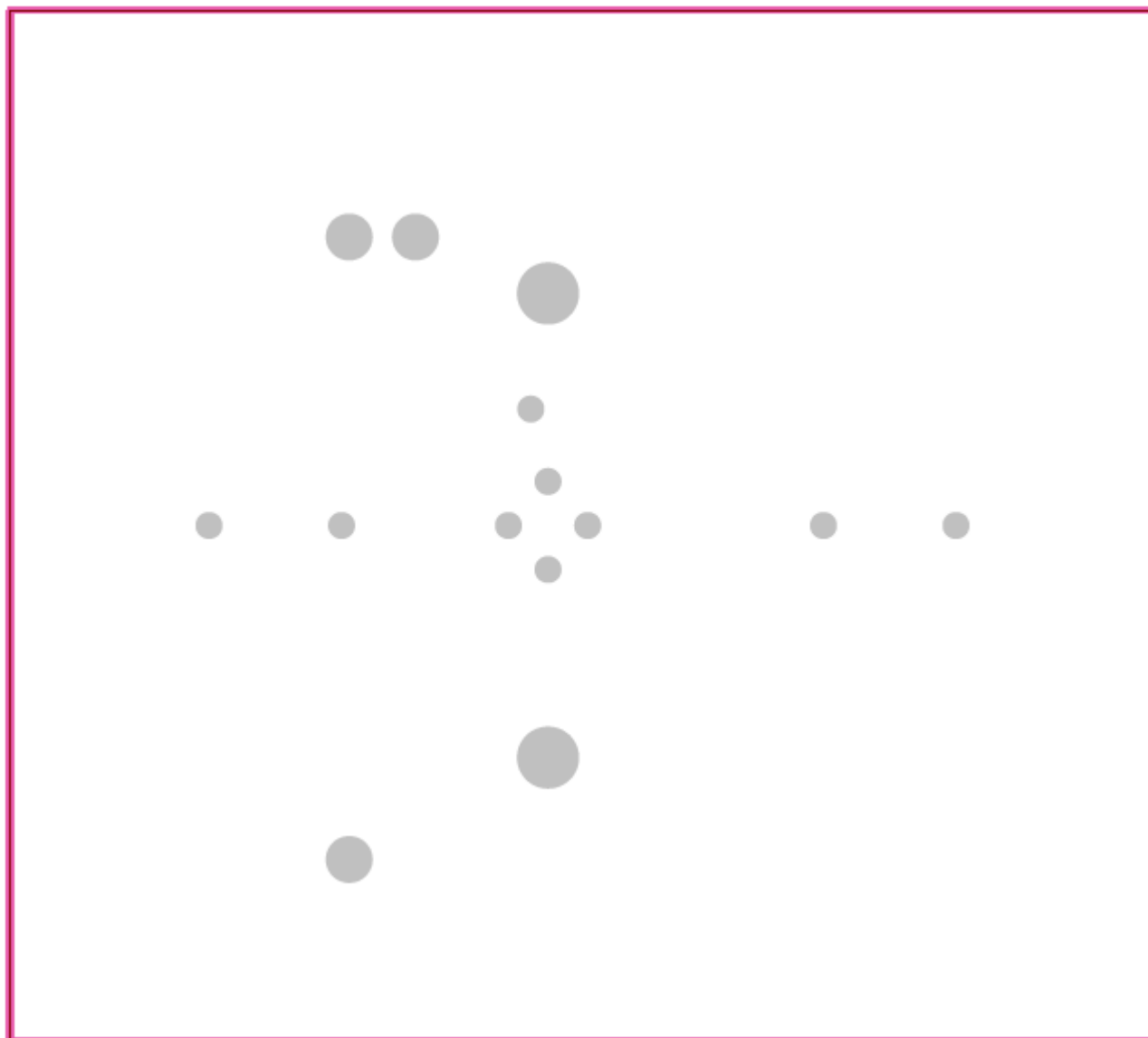
Figure 4. THS4551RUNEVM Layer 3
