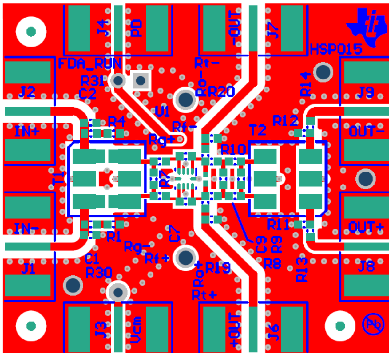
Figure 2. THS4551RUNEVM Top Layer, Signal
