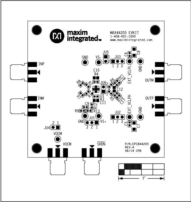
Figure 2. MAX44205 EV Kit Component Placement Guide—Component Side
