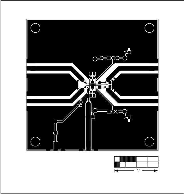
Figure 3. MAX44205 EV Kit PCB Layout—Component Side
