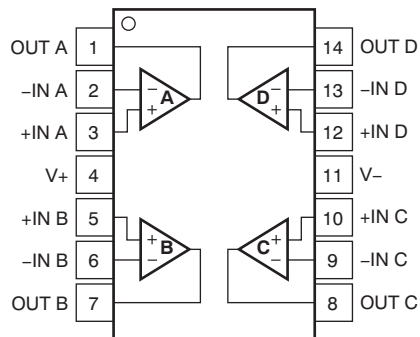
Pin Functions: OPA4180
