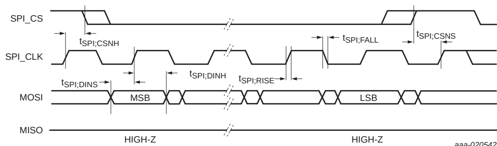
Fig 9. SPI write timing
