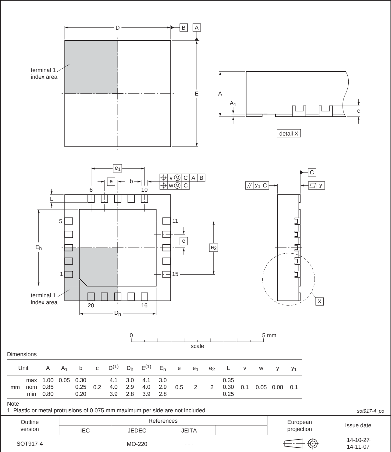
Fig 11. Package outline SOT917-4 (HVQFN20)
