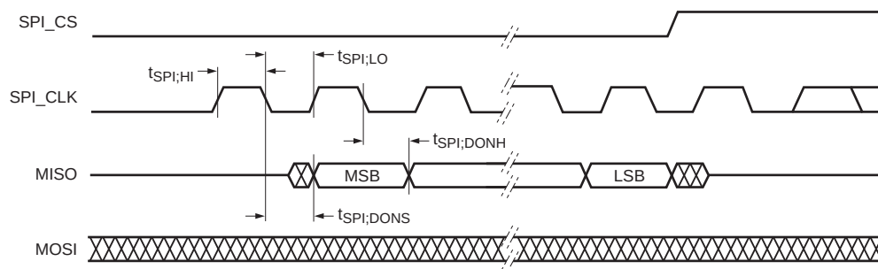
Fig 10. SPI read timing
