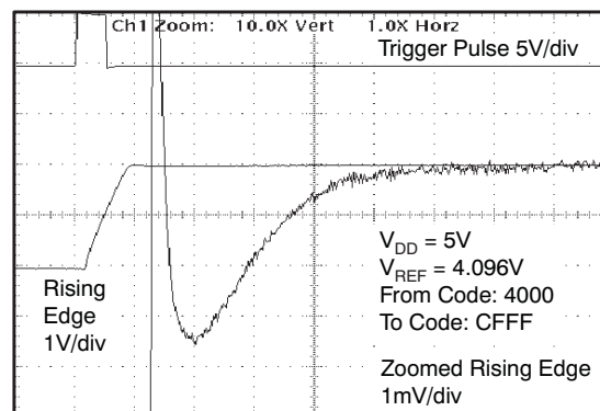
Figure 15. Half-Scale Settling Time, 5-V Rising Edge
