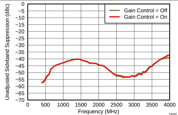
Figure 31. Unadjusted Sideband Suppression vs LO Frequency ( f_{LO} ) and Gain Select Setting
