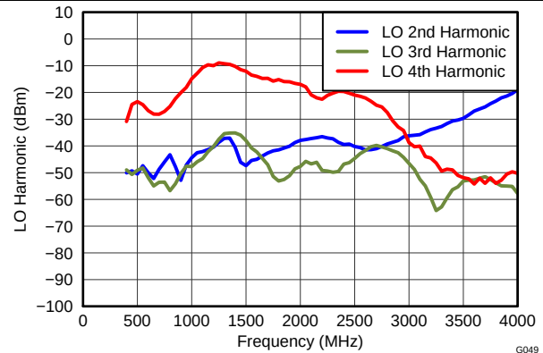
Figure 51. LO Harmonics vs LO Frequency ( f_{LO} )
