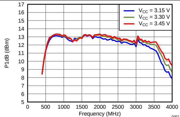
Figure 8. P1dB vs LO Frequency ( f_{LO} ) and Supply Voltage
