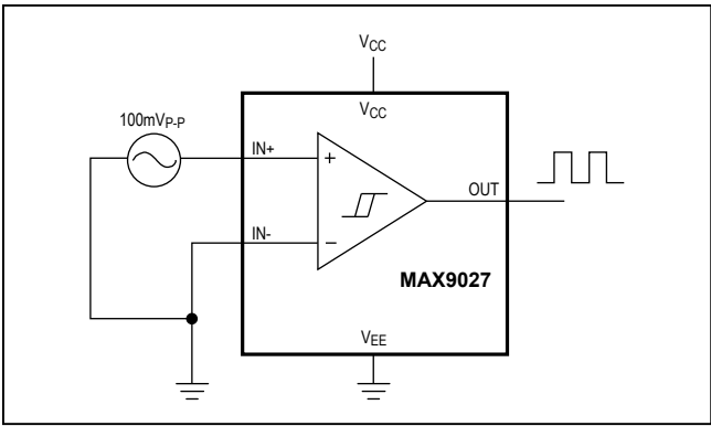
Figure 4. Zero-Crossing Detector
