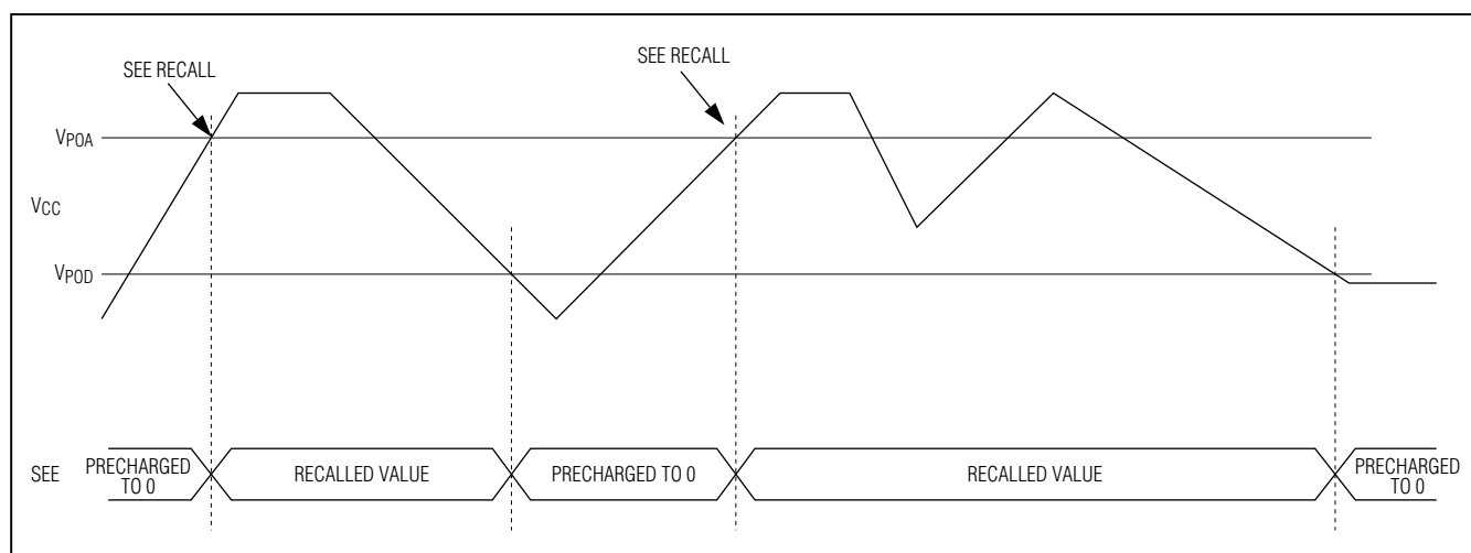
Figure 7. Low-Voltage Operation
