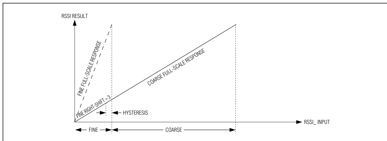
Figure 6. Crossover Disabled
