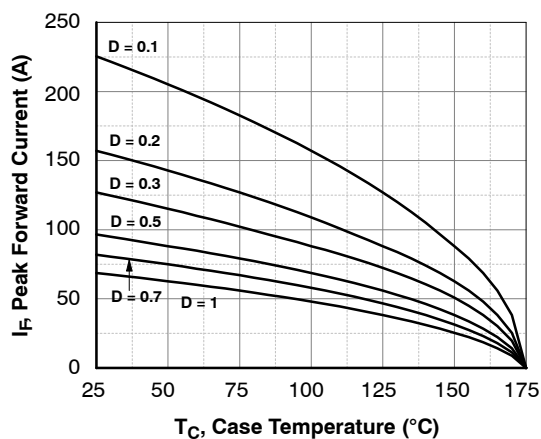
Figure 4. Current Derating
