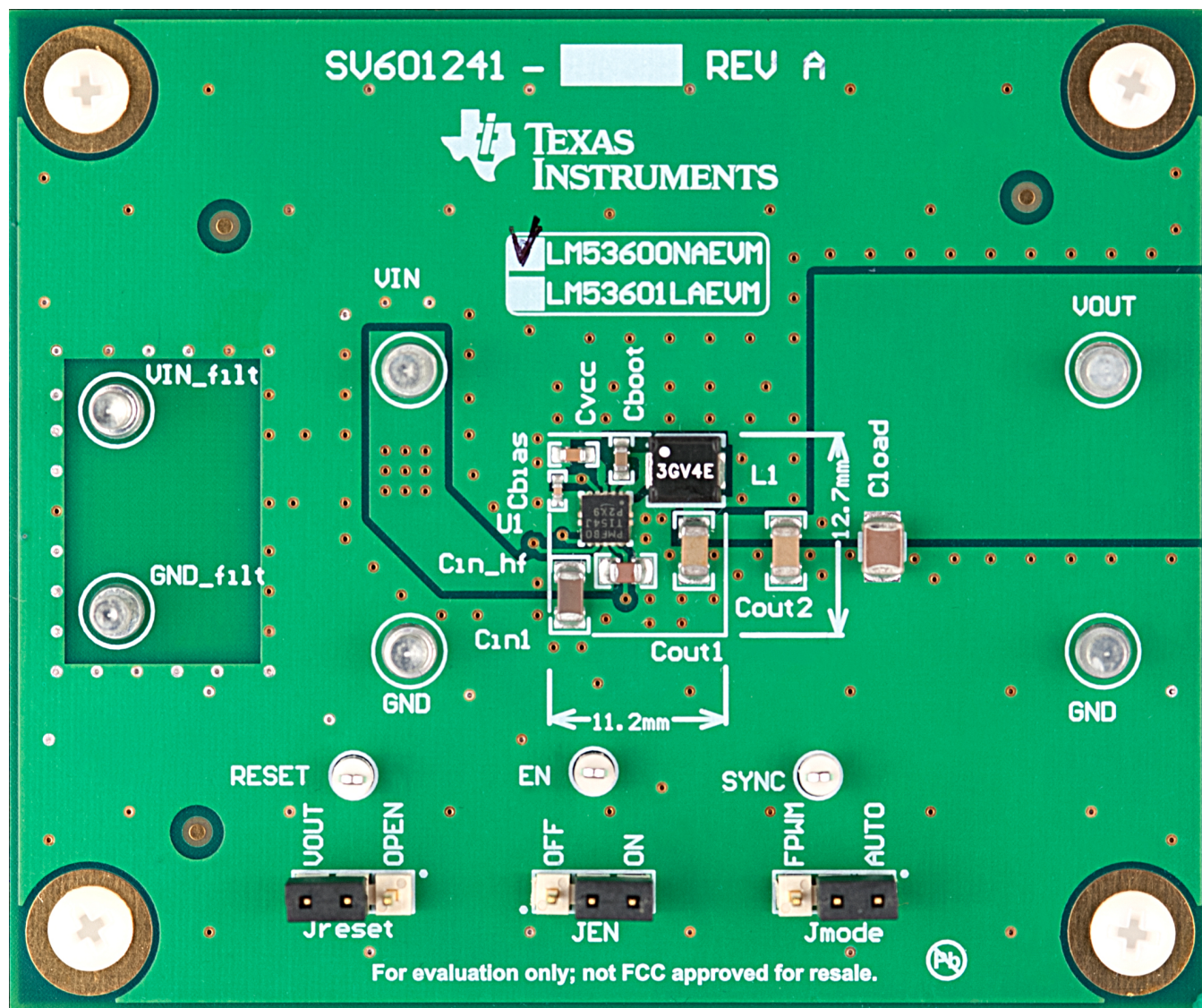
Figure 1-1. LM53600NAEVM
