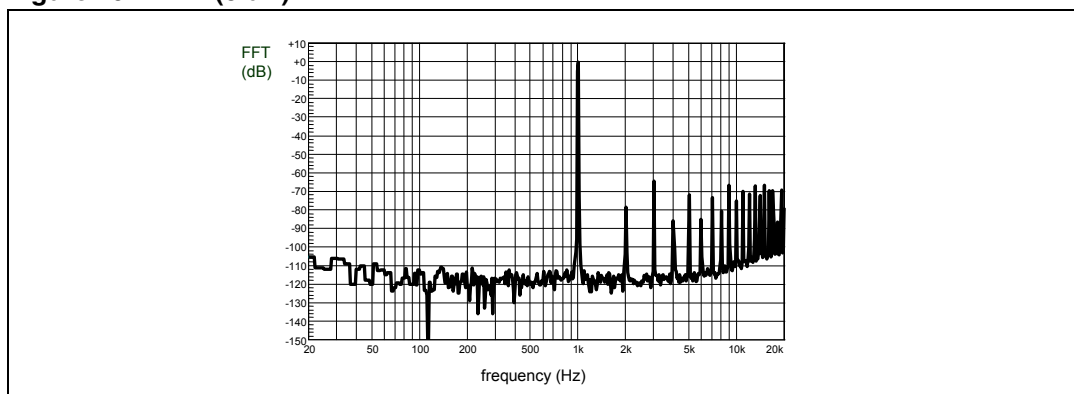
Figure 30. FFT (-60 dB)
