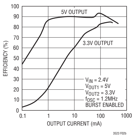
Figure 2. Dual Converter Efficiency (Load Applied to Step-Down Output)
