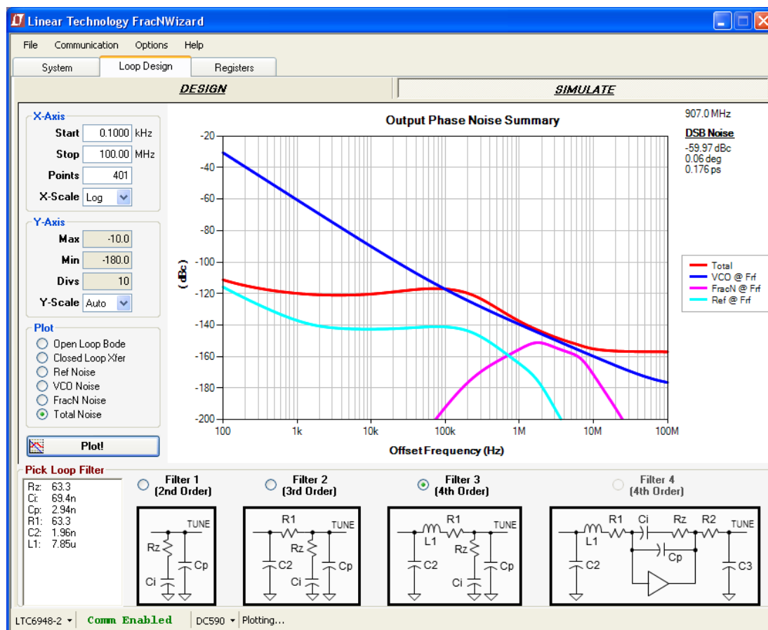
Figure 3. FracNWizard Screenshot
