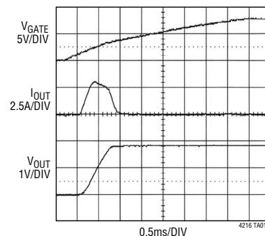
Normal Power-Up with Soft-Start
