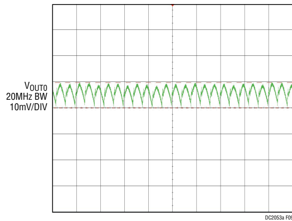
Figure 9. Output Voltage Ripple at V_{IN} = 12V , V_{OUT0} = 1V , I_{OUT0} = 9A
