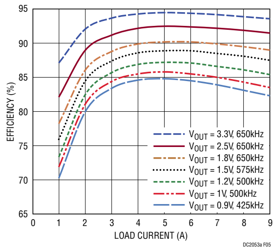
Figure 5. Efficiency vs Load Current at V_{IN} = 5V
