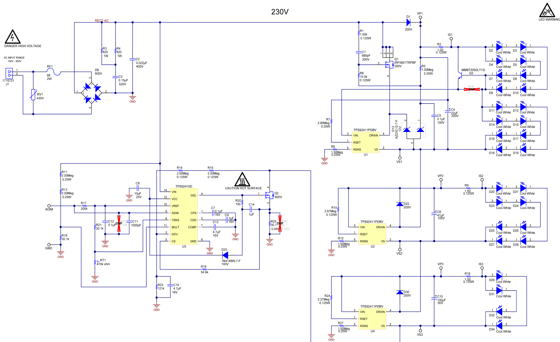
Figure 1. TPS92410EVM-002 Schematic
