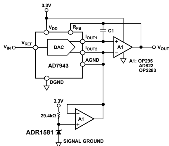
Figure 25. Single-Supply System
