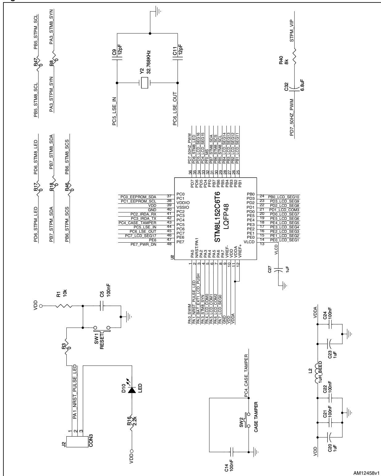
Figure 8. Microcontroller schematic
