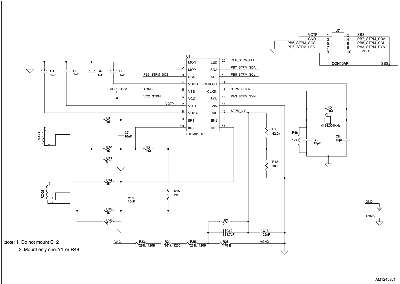
Figure 11. STPM schematic
