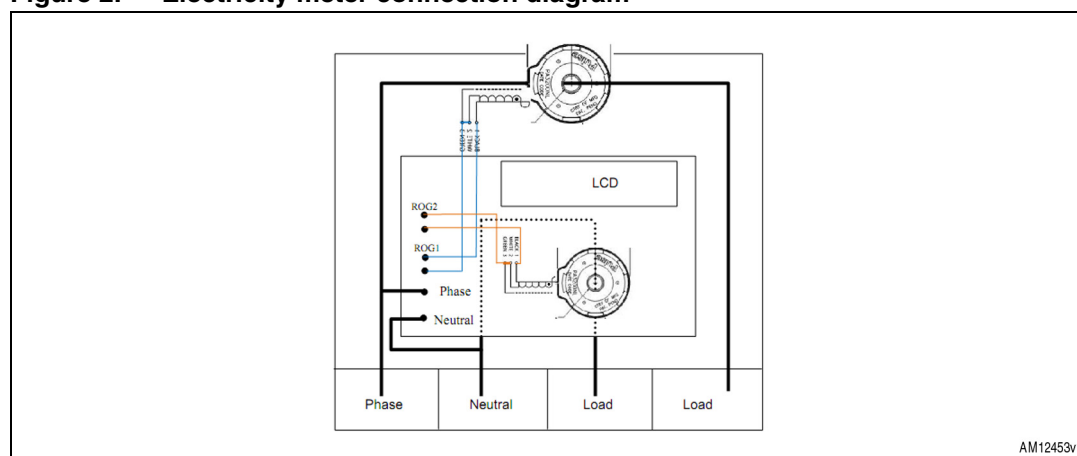
Figure 2. Electricity meter connection diagram
