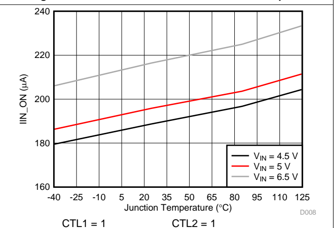
Figure 8. Enabled IN Supply Current – CDP (11) vs Temperature
