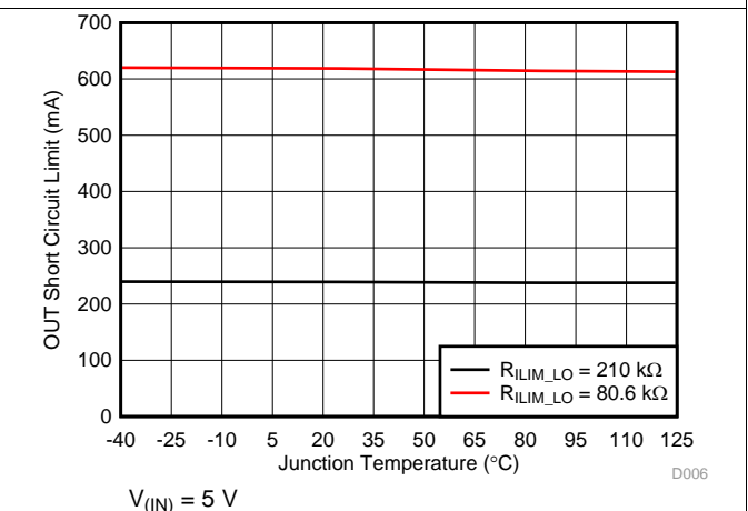
Figure 6. OUT Short-Circuit Current Limit vs Temperature II
