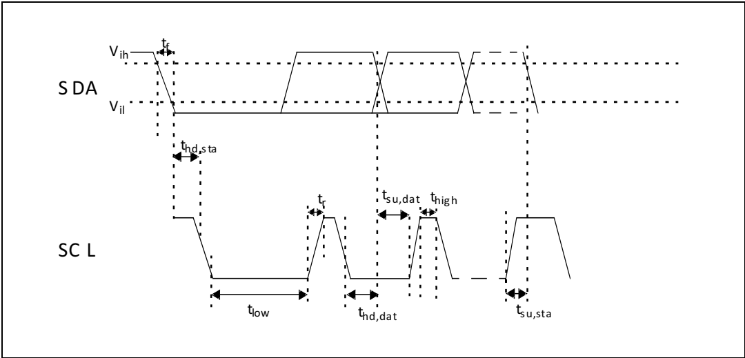
Figure 7. I²C timing diagram
