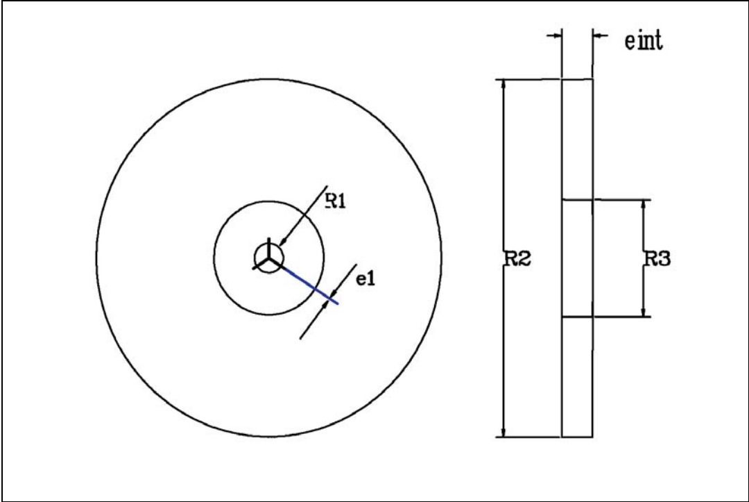
Figure 13. Reel information
