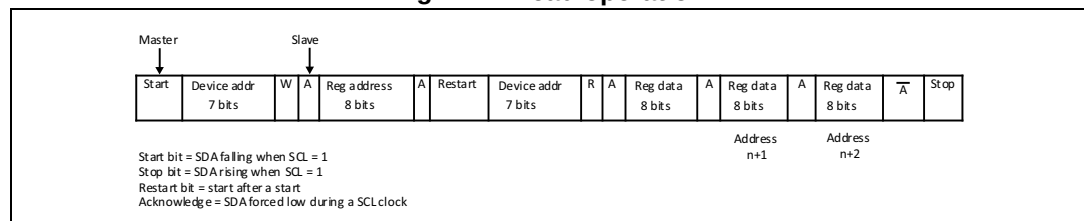
Figure 5. Read operation
