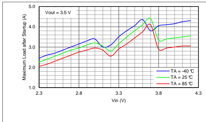
Figure 26. Maximum Load Current after Startup
