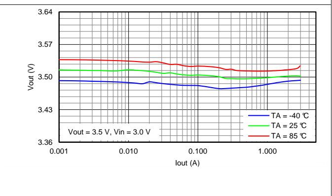
Figure 29. Load Regulation
