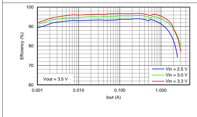
Figure 28. Efficiency
