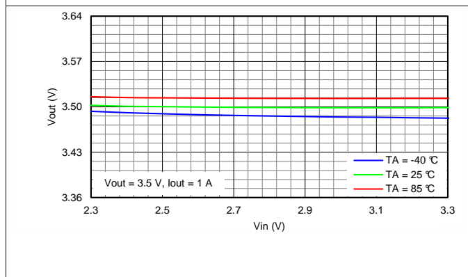
Figure 30. Line Regulation
