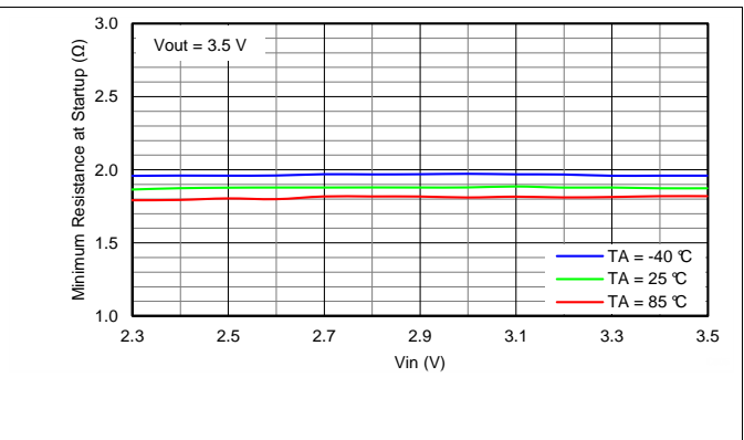
Figure 27. Minimum Resistance at Startup
