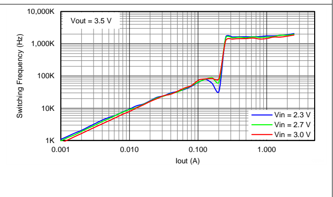
Figure 31. Switching Frequency
