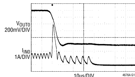
FIGURE 69 CIRCUIT AT 12\text{V}_{\text{IN}} , 77\text{m}\Omega LOAD ON \text{VOUT}_0 PRIOR TO APPLICATION OF SHORT CIRCUIT
