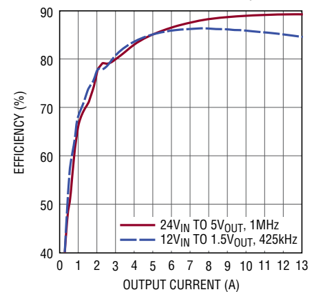
Single Phase Single Output Pulse-Skipping (Discontinuous) Mode Efficiency, \text{V}_{\text{IN}} = \text{SV}_{\text{IN}} = \text{V}_{\text{INn}} , \text{INTV}_{\text{CC}} Open, \text{MFR\_PWM\_MODE}_n[0] = 0_b
