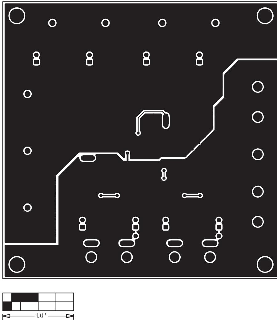
Figure 4. MAX4079 EV Kit PCB Layout—Solder Side
