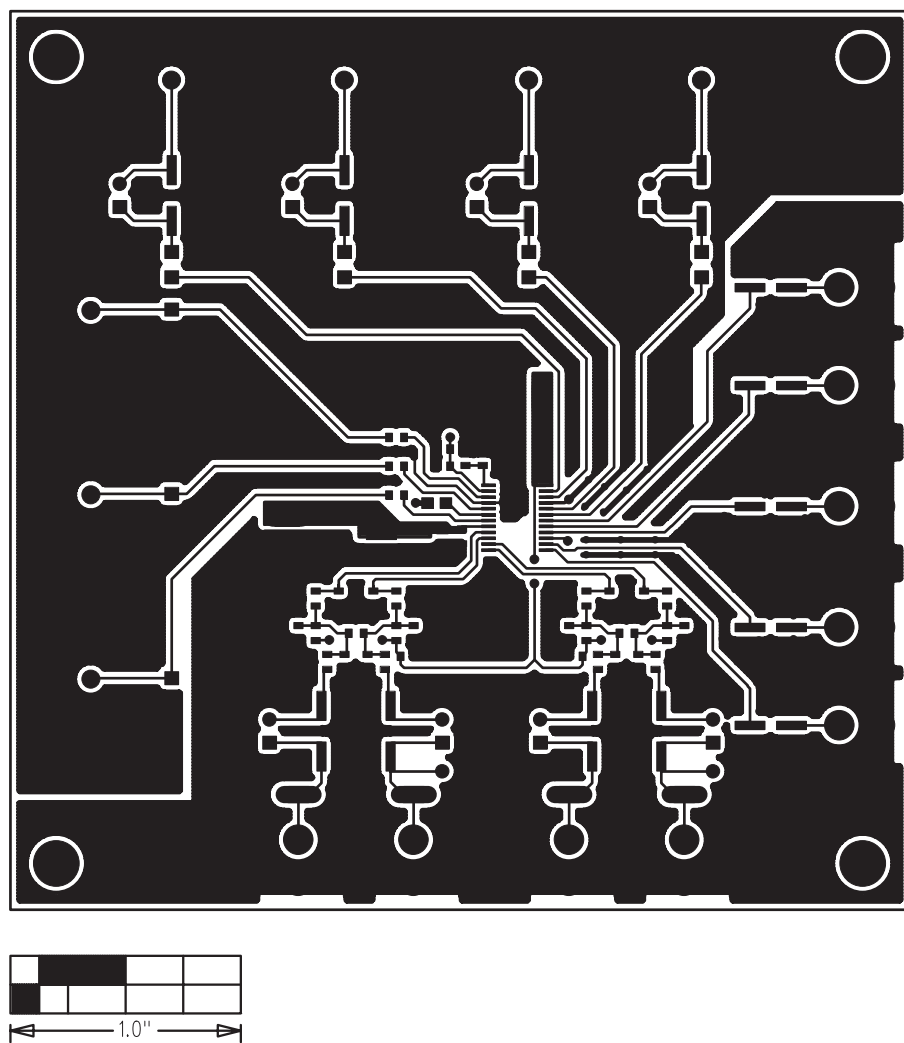
Figure 3. MAX4079 EV Kit PCB Layout—Component Side
