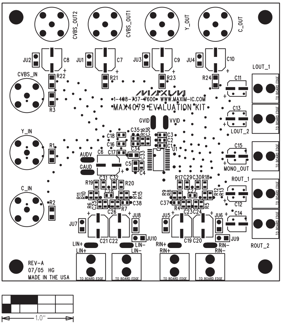
Figure 2. MAX4079 EV Kit Component Placement Guide—Component Side
