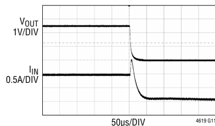
Short Circuit, I_{OUT} = 4\text{A}
