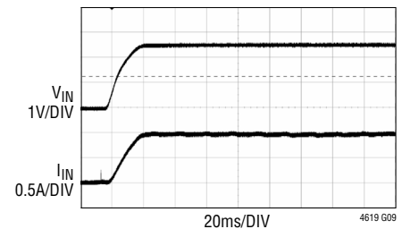
Start-Up, I_{OUT} = 4\text{A}
