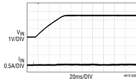
Start-Up, I_{OUT} = 0\text{A}
