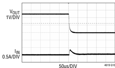
Short Circuit, I_{OUT} = 0\text{A}
