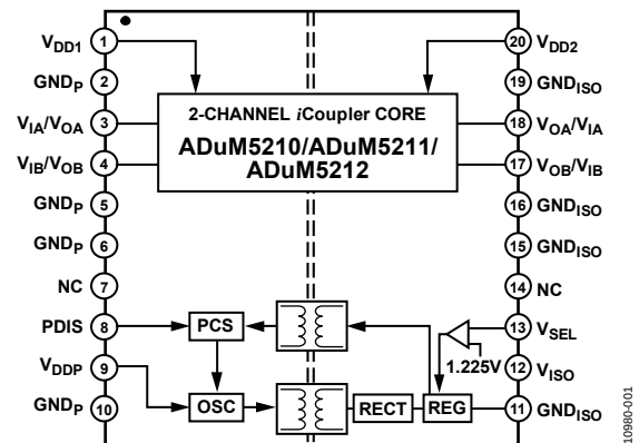
Figure 1. ADuM5210/ADuM5211/ADuM5212
