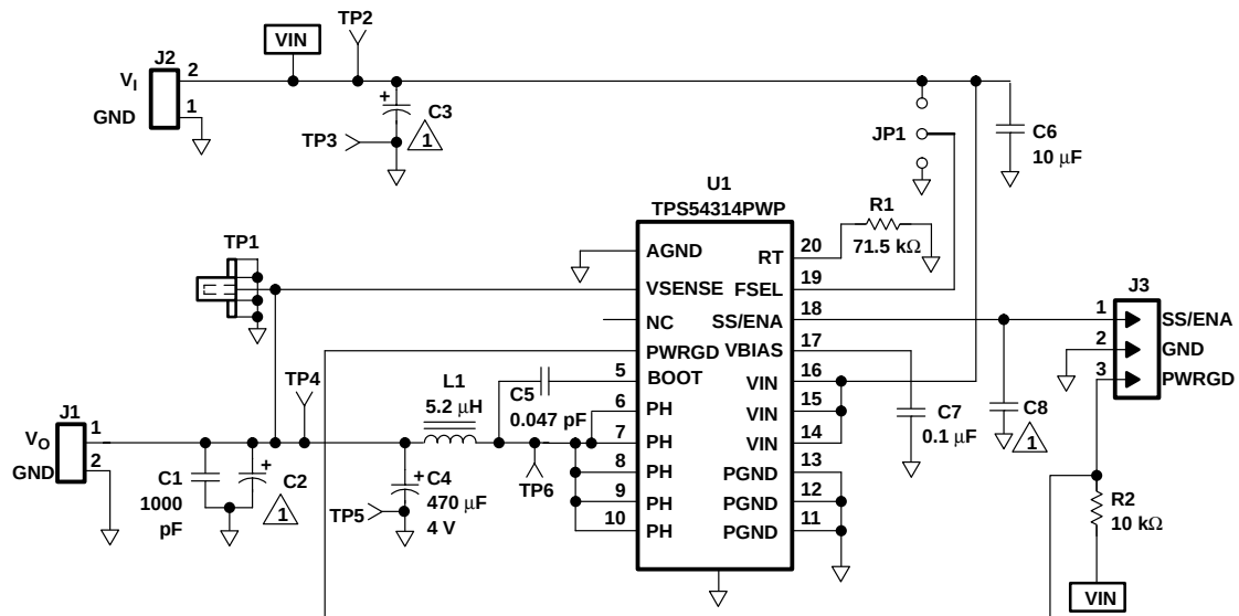
Figure 4–1. TPS54314EVM Schematic
