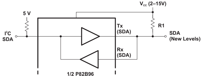
Figure 15. Interfacing I 2 C Bus With Different Logic Levels
