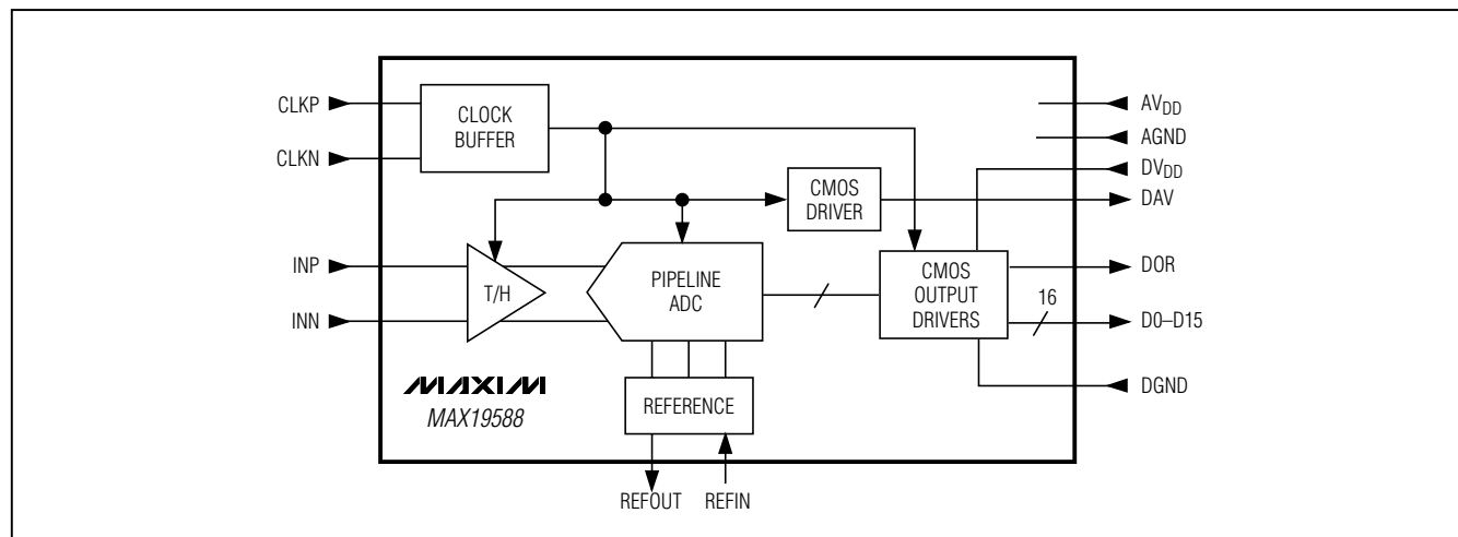
Figure 1. Block Diagram
