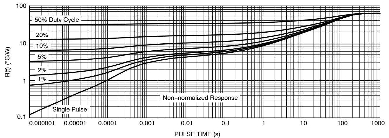
Figure 27. Duty Cycle for 1 inch² (645 mm²) Spreader Board, DPAK 3-Lead
