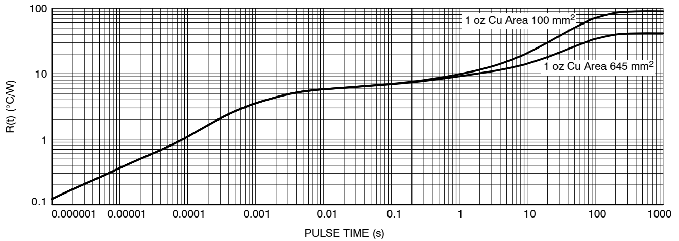
Figure 25. Single-Pulse Heating Curves, D²PAK 3-Lead
