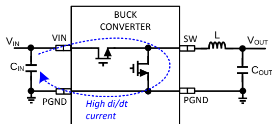
Figure 97. Buck Converter High \Delta i/\Delta t Path
