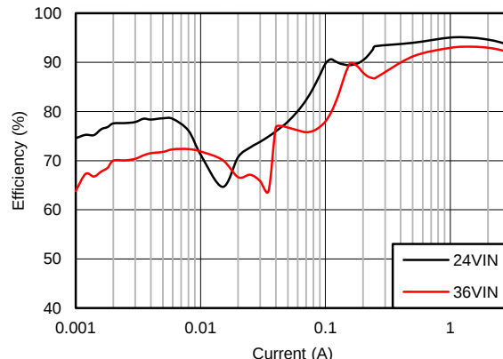
Figure 92. Efficiency
