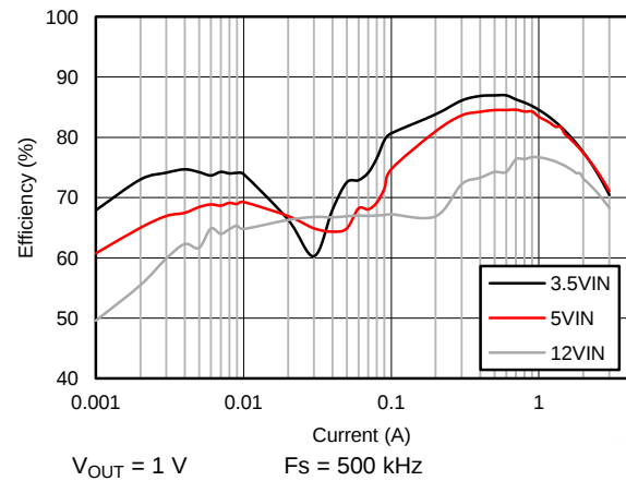
Figure 50. Efficiency
