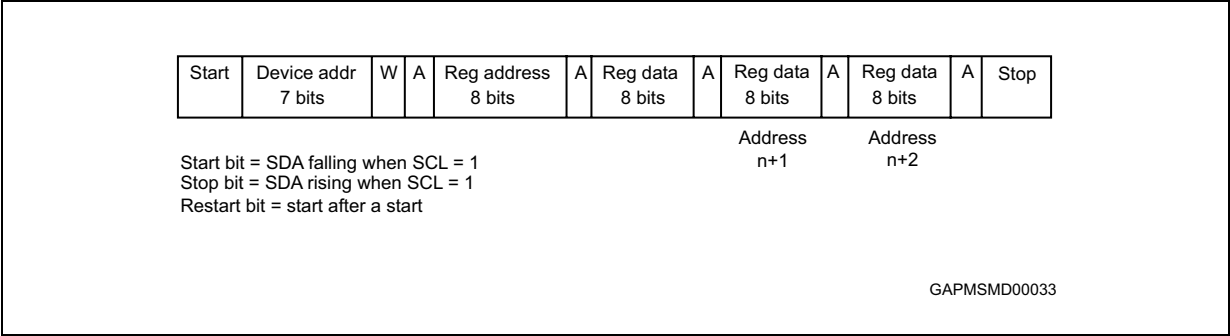
Figure 14. Write operation
