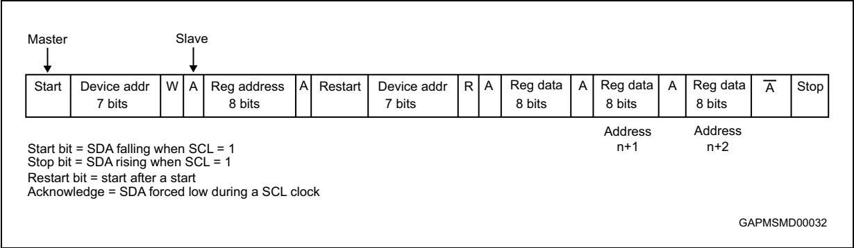
Figure 13. Read operation
