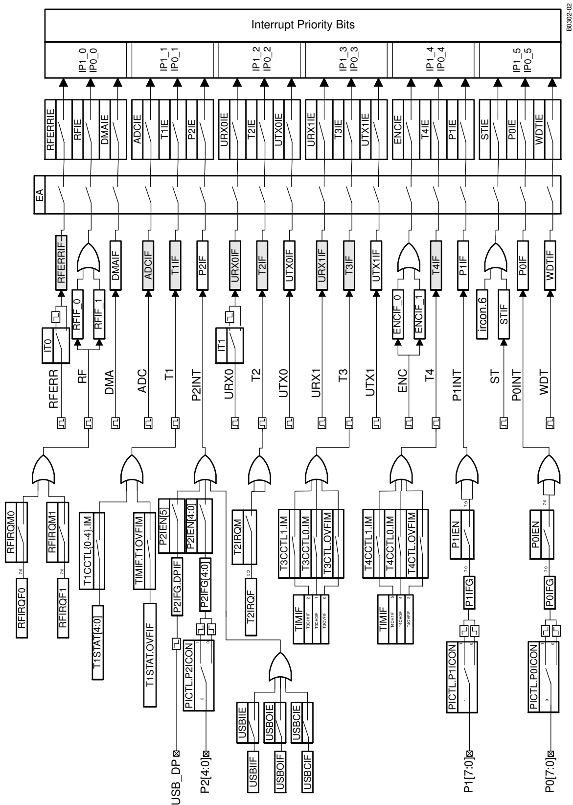
Figure 2-4. Interrupt Overview
