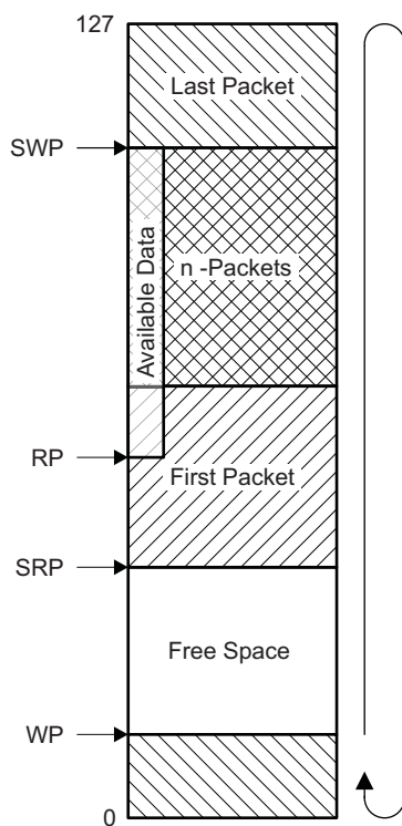
Figure 25-2. FIFO Pointers
