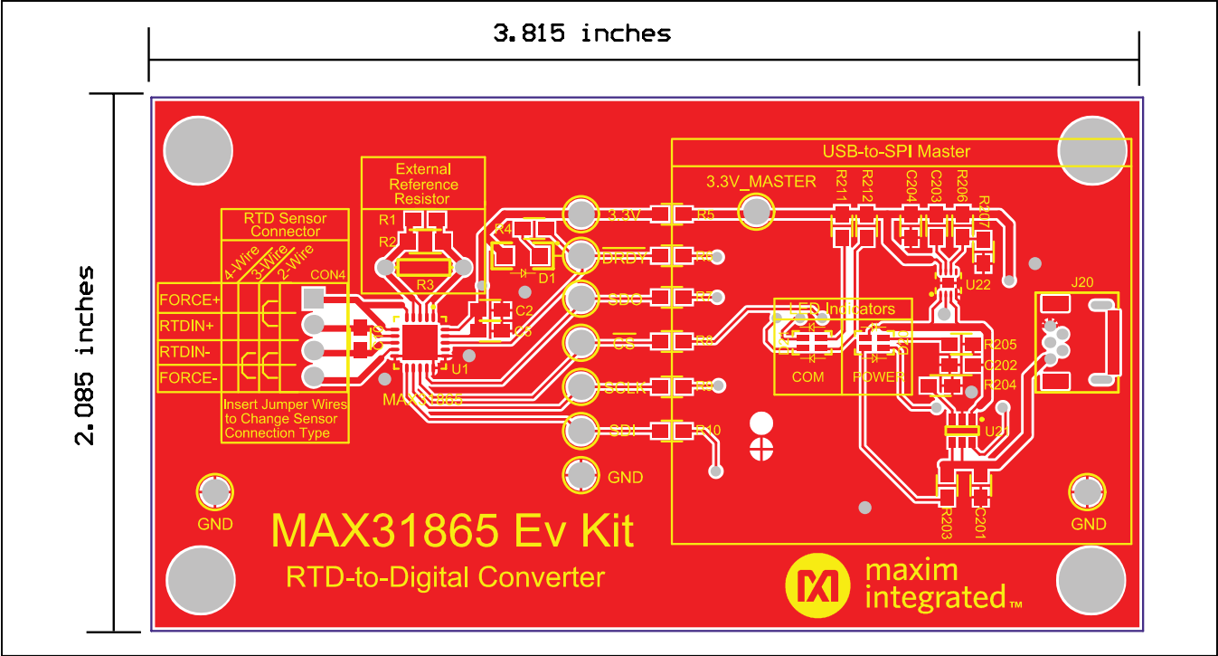
Figure 6. MAX31865 EV Kit PCB Layout—Top
