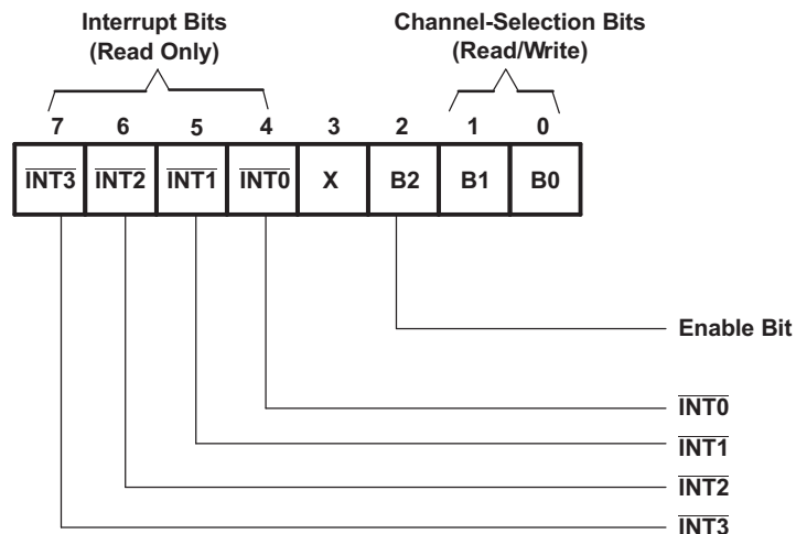
Figure 10. Control Register
