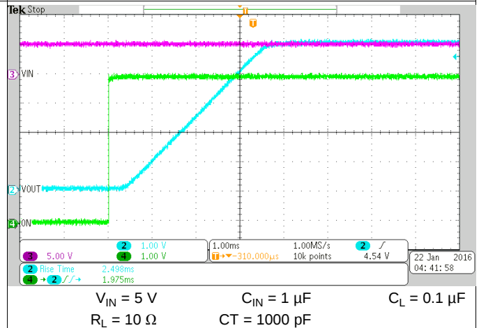
Figure 13. Rise Time ( t_R ) at V_{IN} = 5\text{ V}
