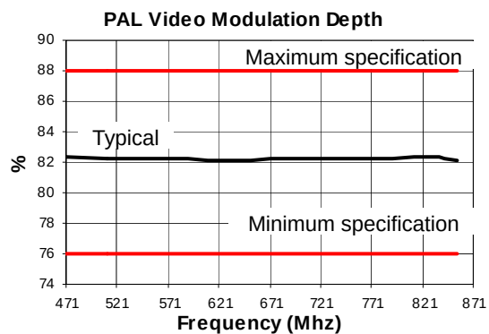
Figure 4. Typical Video Performance
