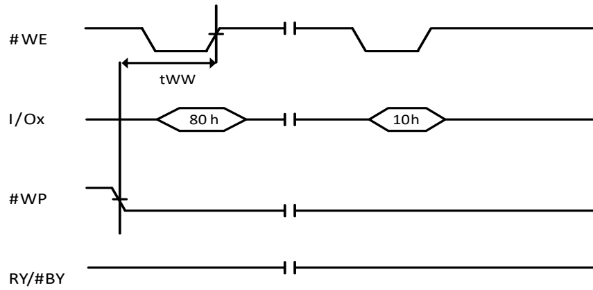
Figure 9-15 Program Disable
