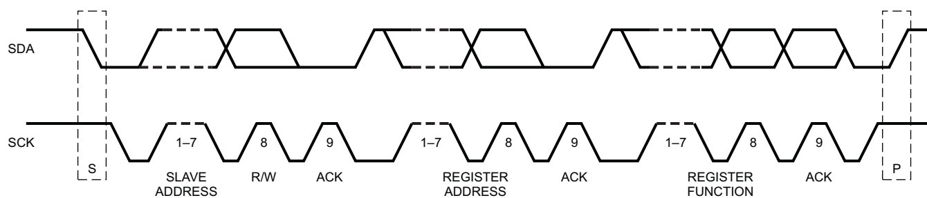
Figure 3. I²C Data Transfer
