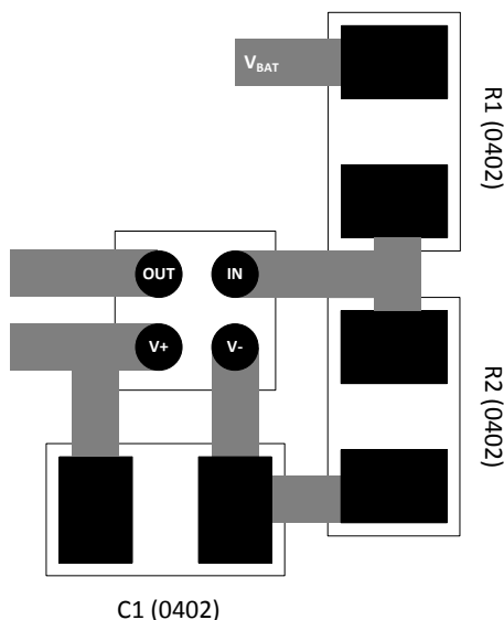
Figure 46. Layout Example
