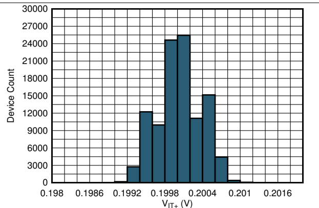
Figure 9. Positive Threshold Histogram
