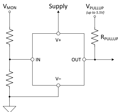
Figure 43. Level-Shifting
