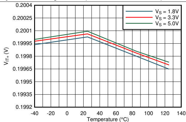
Figure 8. Positive Threshold vs Temperature
