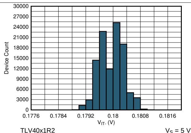
Figure 11. Negative Threshold Histogram
